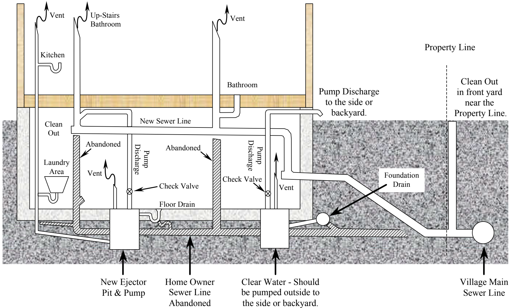
Section Thru Basement
